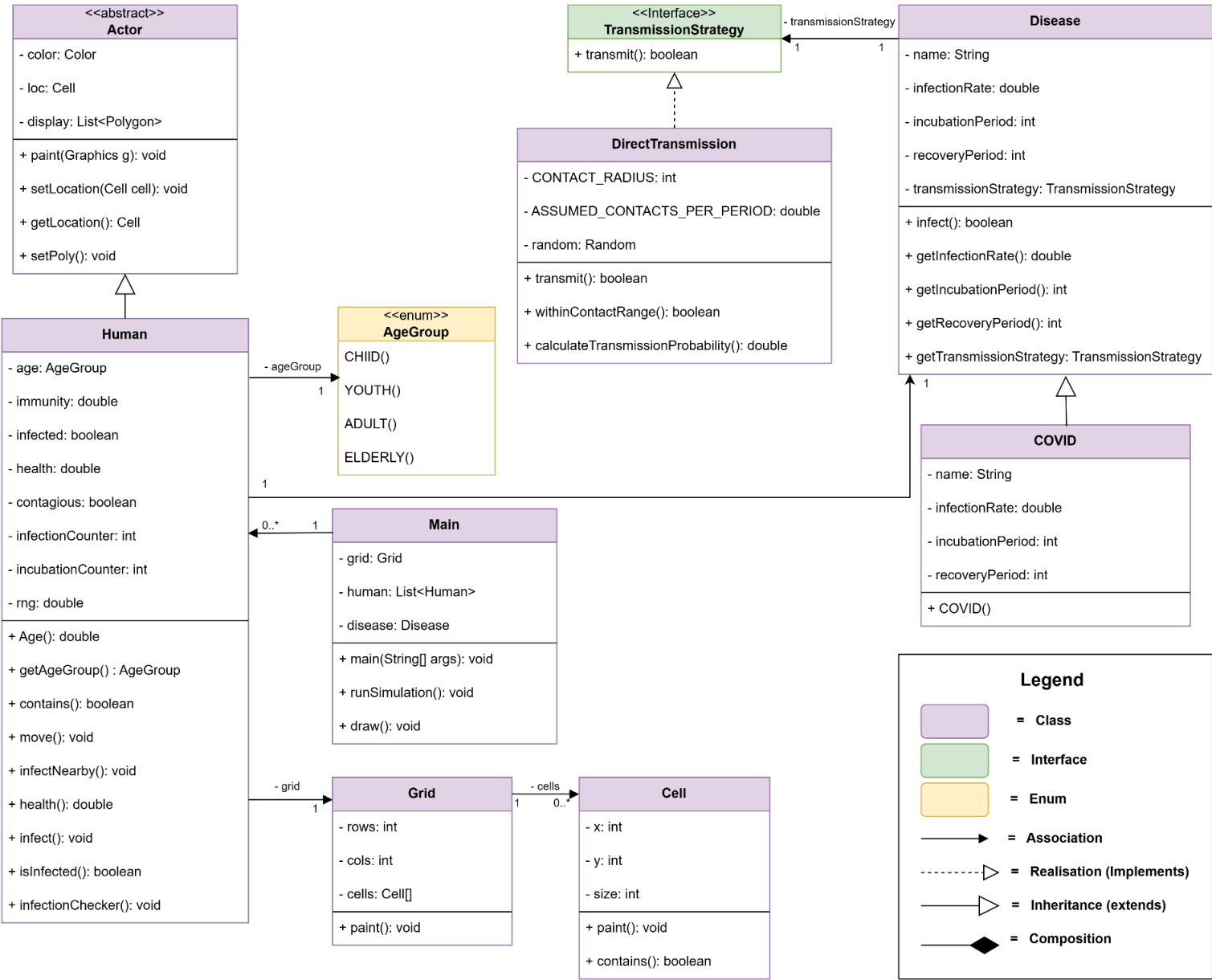
Epidemic Spread Simulation - UML Class Diagram (Final Design)
